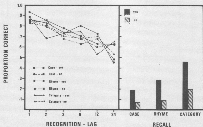
FIG. 4. Initial recognition (left panel) and final free recall (right panel) in a "levels-of-processing" task.
